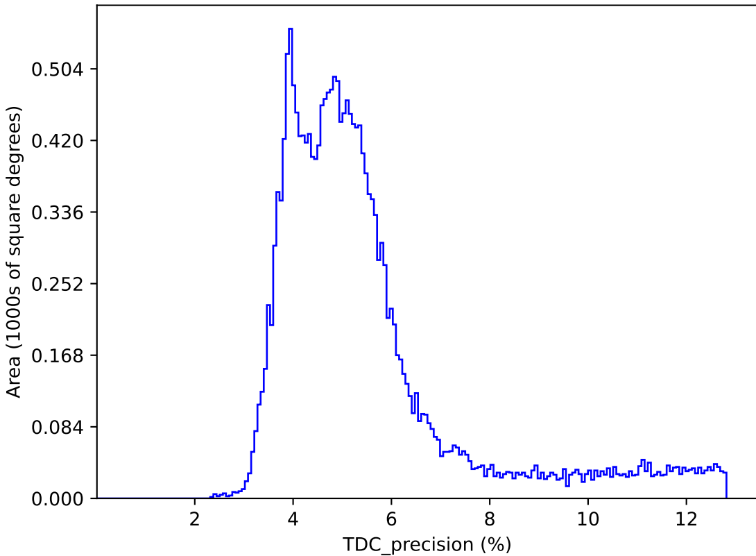
too_elab_r128_d2_griz_v3.4_10yrs : TDC_precision
