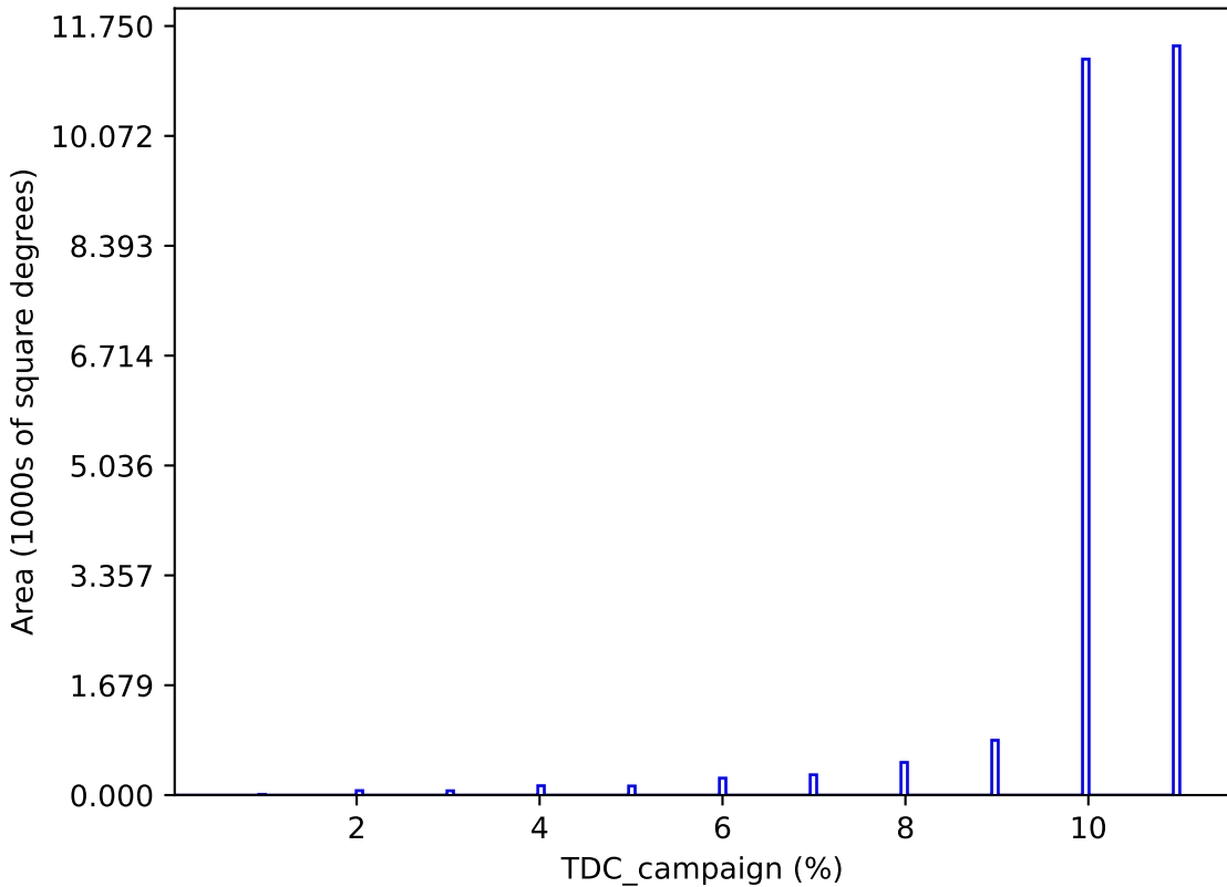
too_elab_r128_d2_griz_v3.4_10yrs : TDC_campaign
