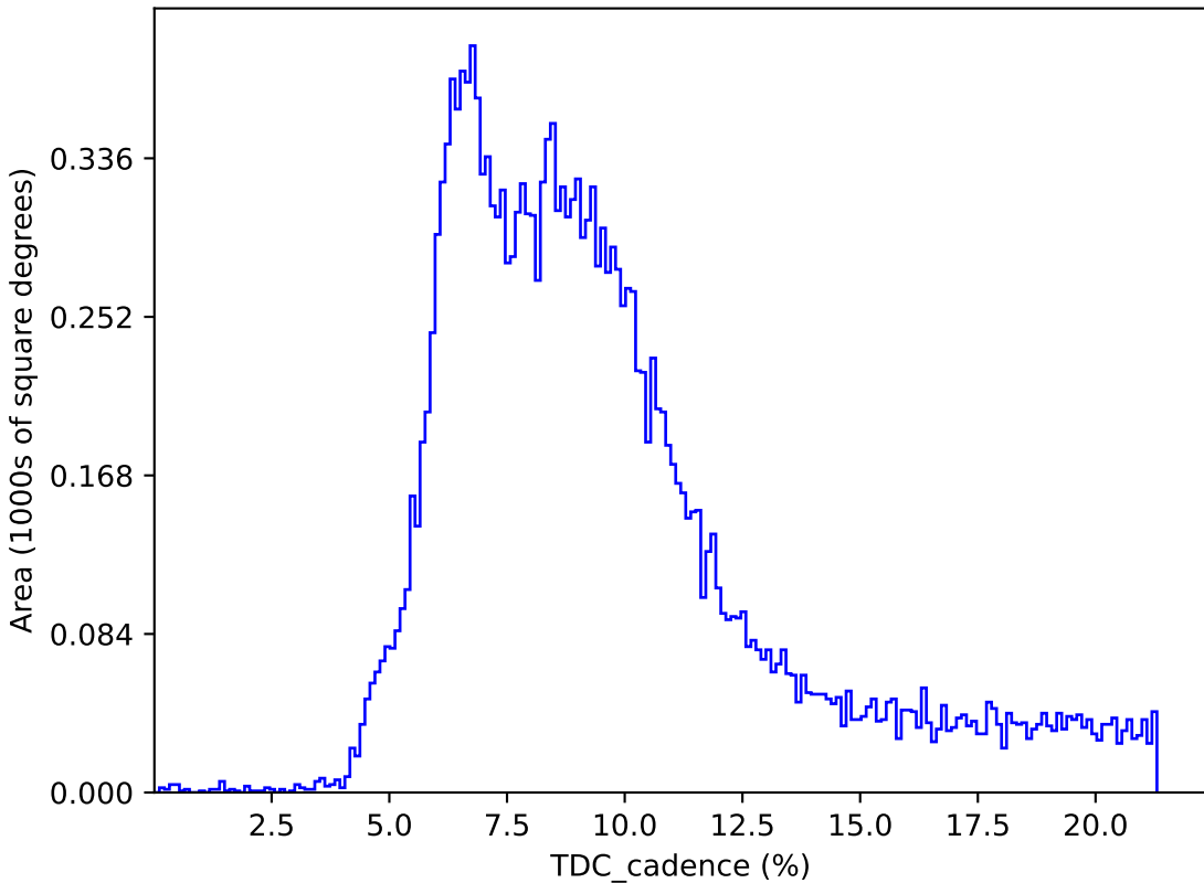
too_elab_r128_d2_griz_v3.4_10yrs : TDC_cadence
