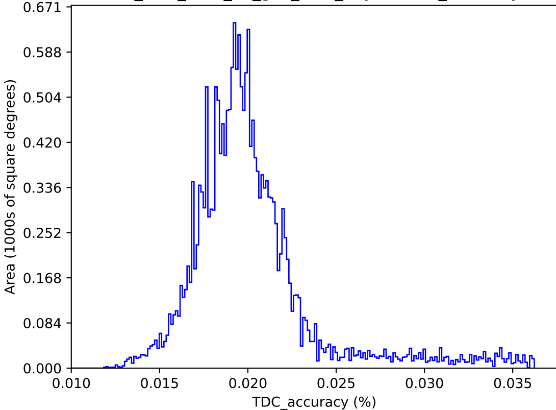
too_elab_r128_d2_griz_v3.4_10yrs : TDC_accuracy
