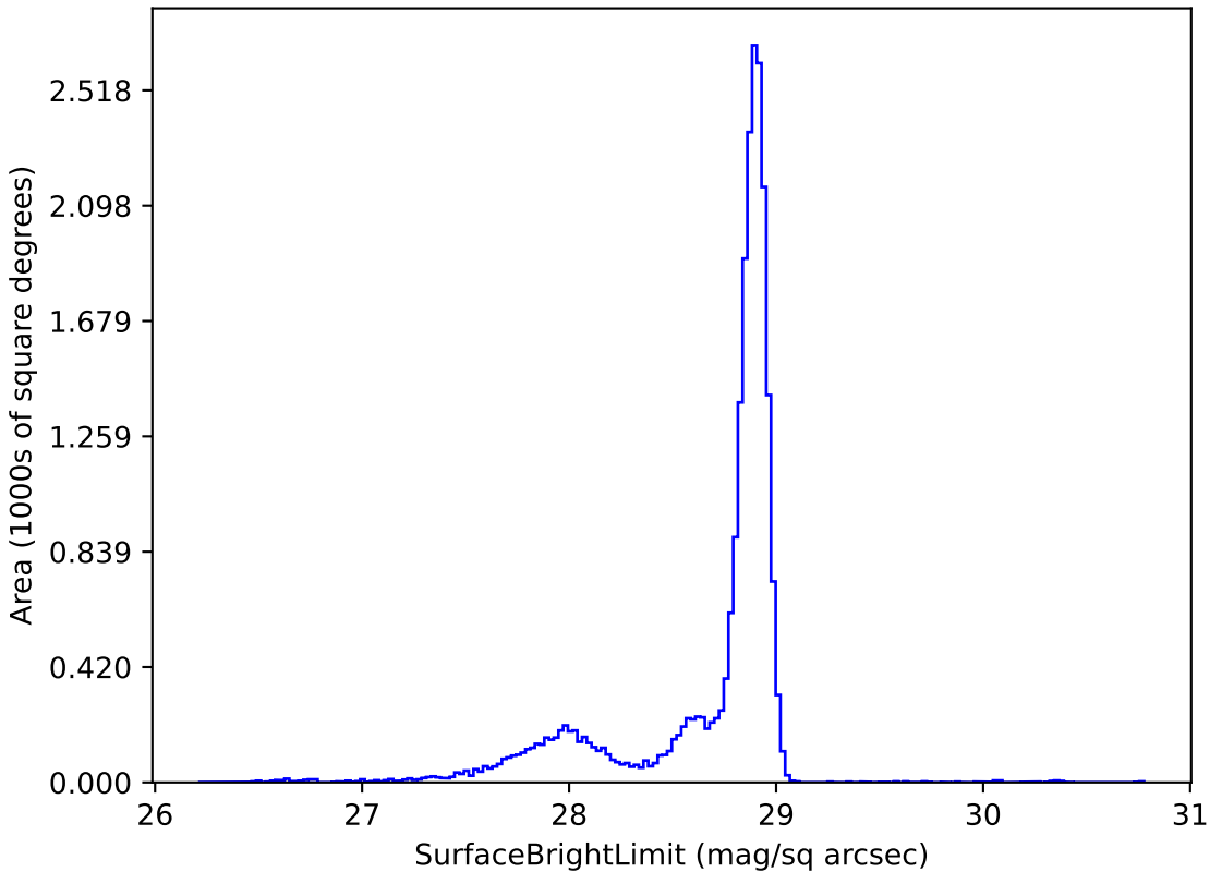
too_elab_r128_d2_griz_v3.4_10yrs u: SurfaceBrightLimit
