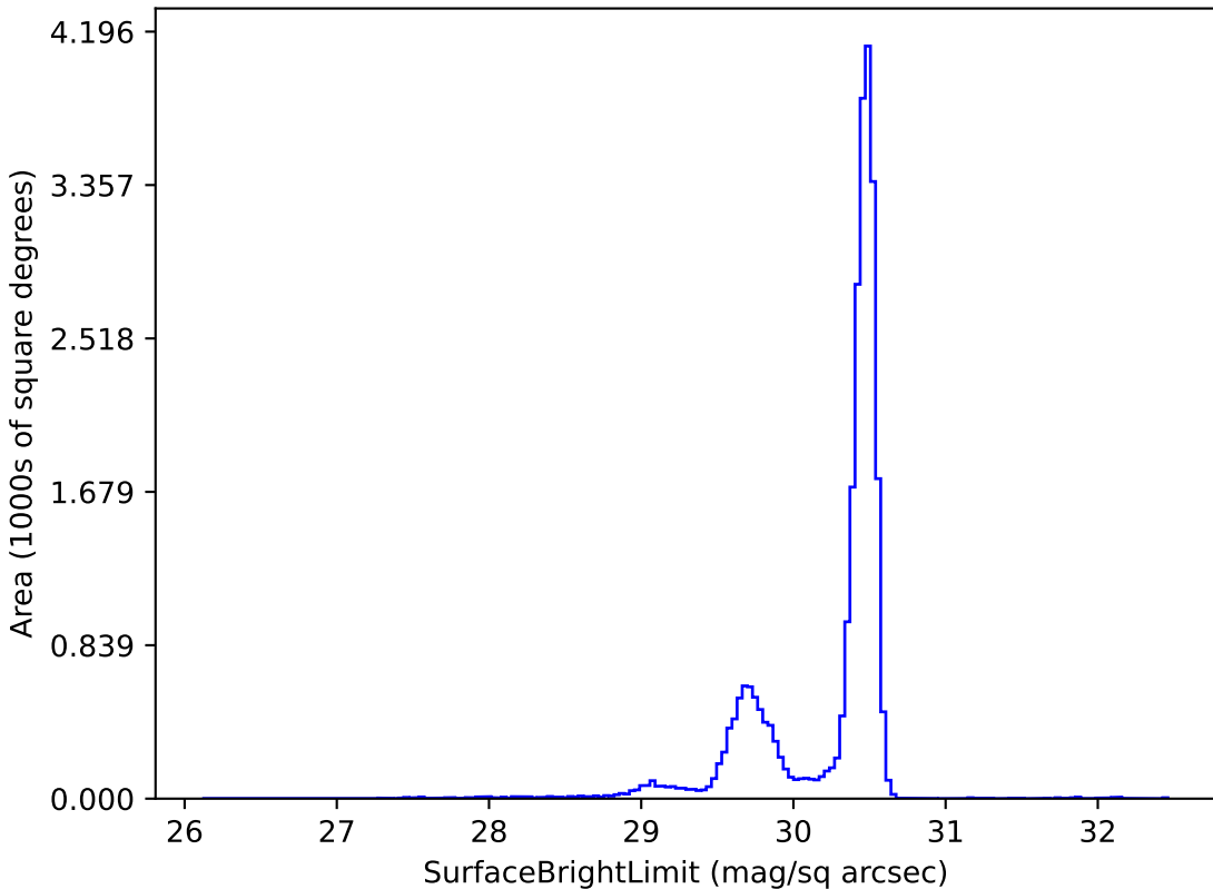
too_elab_r128_d2_griz_v3.4_10yrs r: SurfaceBrightLimit
