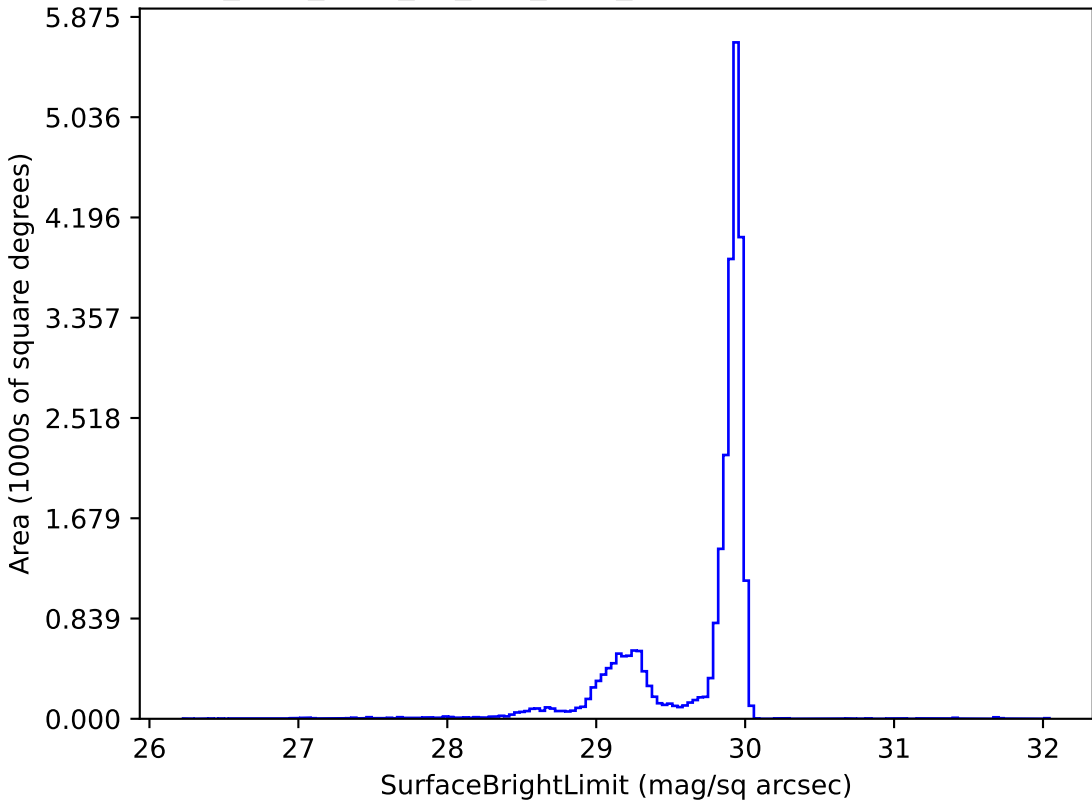
too_elab_r128_d2_griz_v3.4_10yrs i: SurfaceBrightLimit
