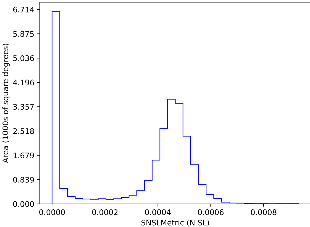
too_elab_r128_d2_griz_v3.4_10yrs : SNSLMetric
