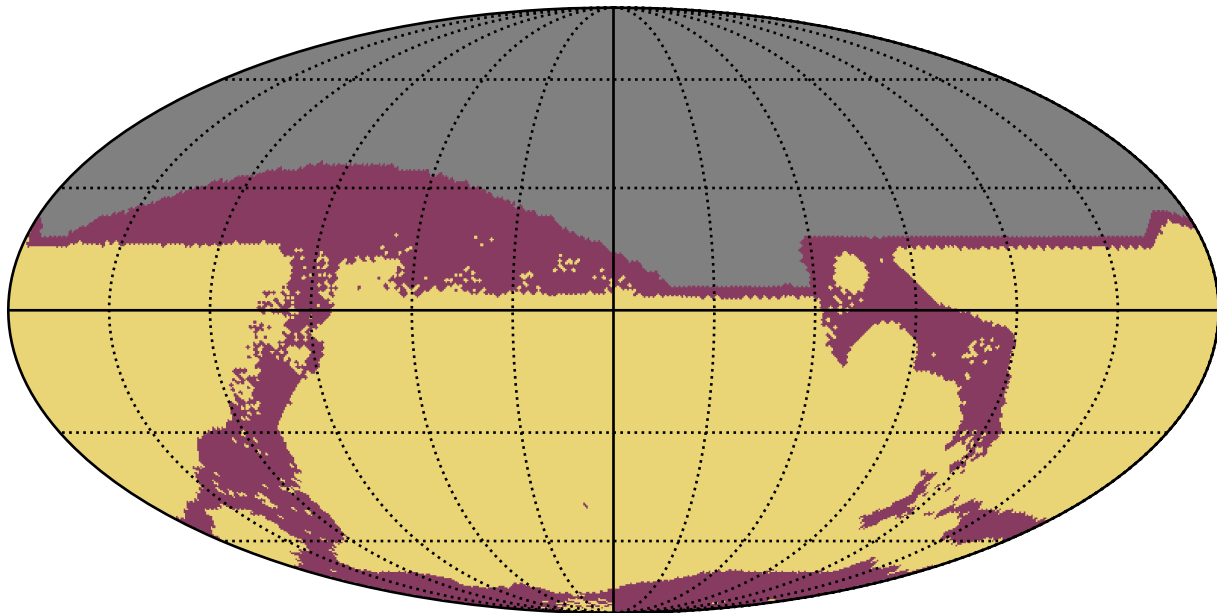
too_elab_r128_d2_griz_v3.4_10yrs : RapidRevisits
