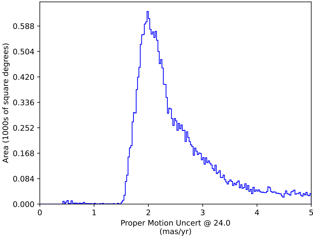
too_elab_r128_d2_griz_v3.4_10yrs : Proper Motion Uncert @ 24.0
