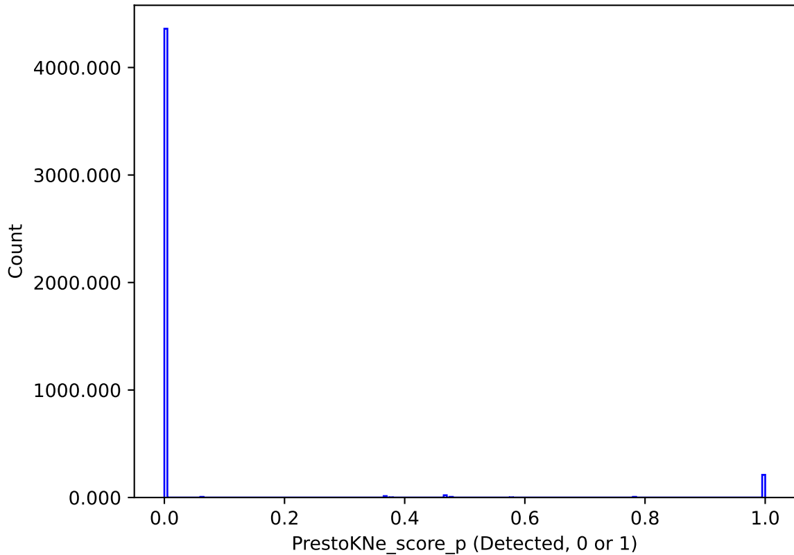
too_elab_r128_d2_griz_v3.4_10yrs : PrestoKNe_score_p
