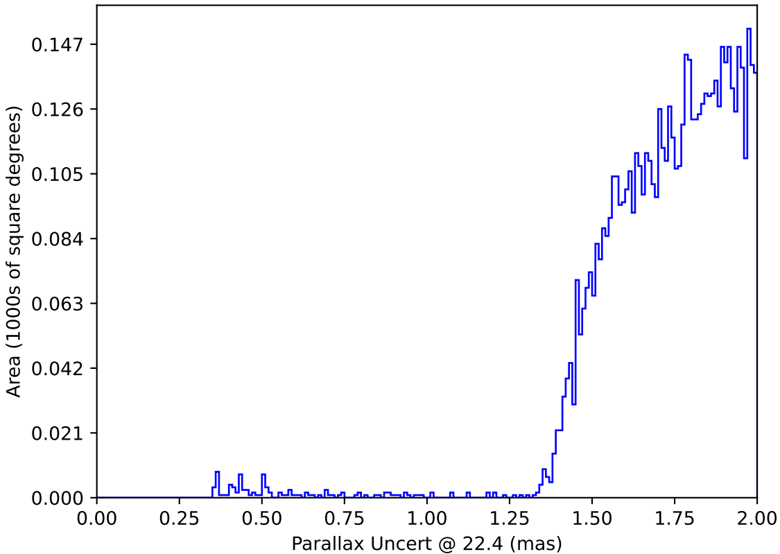
too_elab_r128_d2_griz_v3.4_10yrs : Parallax Uncert @ 22.4
