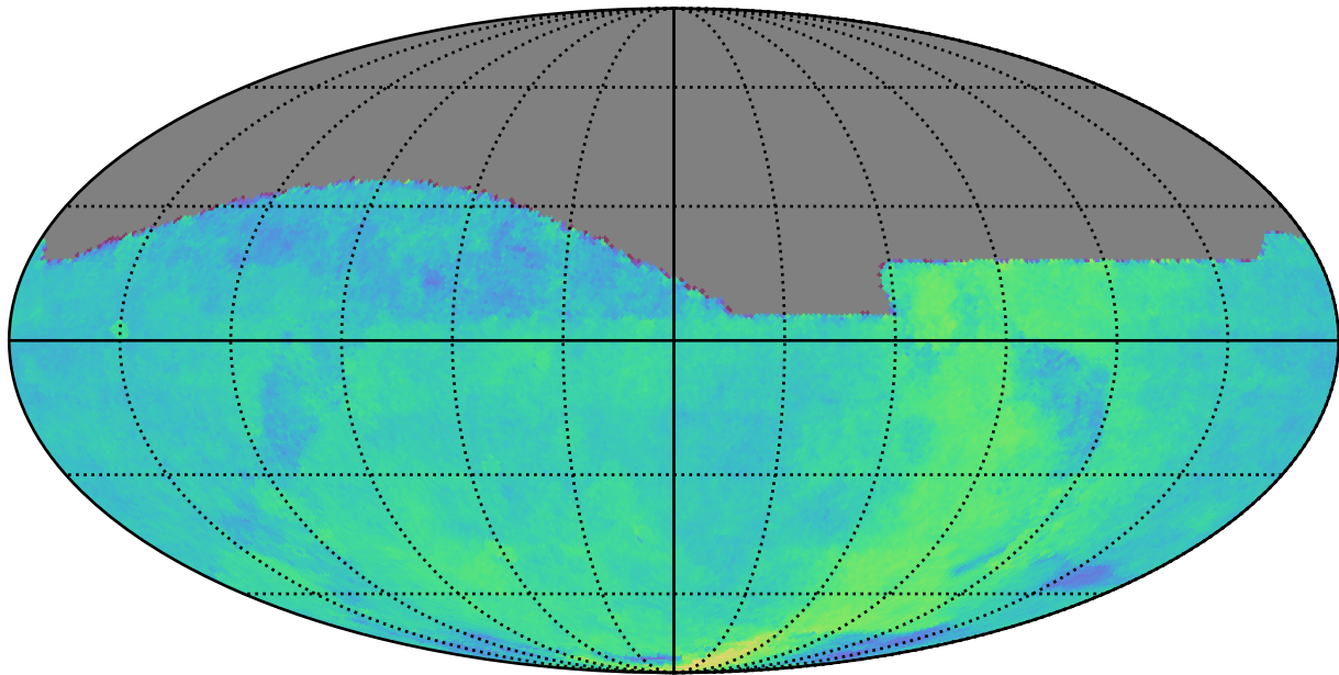
too_elab_r128_d2_griz_v3.4_10yrs : Parallax Coverage @ 22.4
