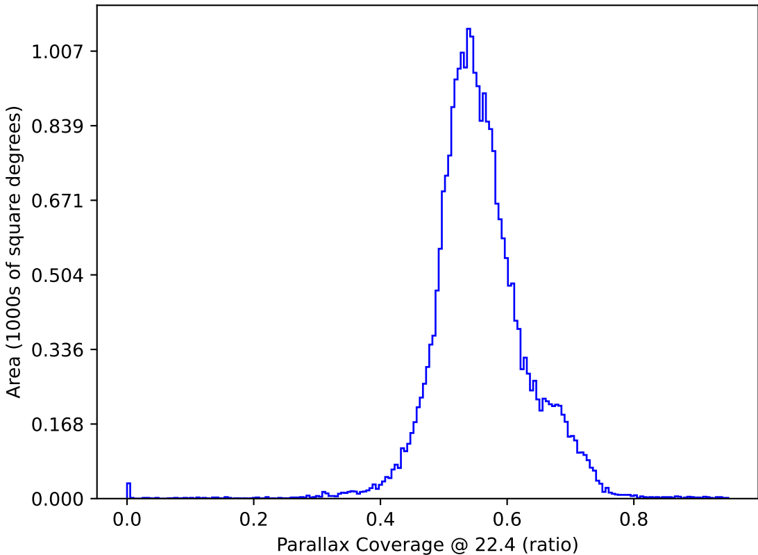
too_elab_r128_d2_griz_v3.4_10yrs : Parallax Coverage @ 22.4
