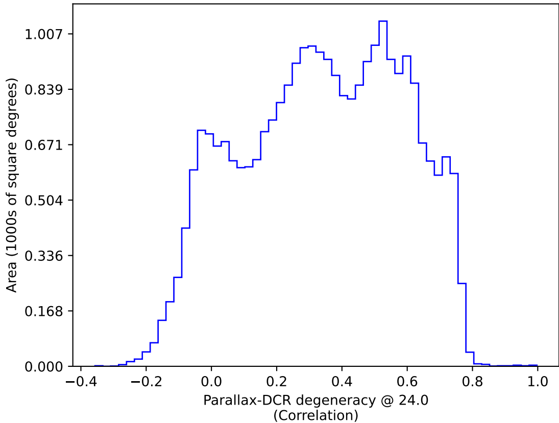
too_elab_r128_d2_griz_v3.4_10yrs : Parallax-DCR degeneracy @ 24.0
