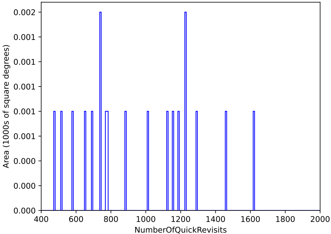
too_elab_r128_d2_griz_v3.4_10yrs : NumberOfQuickRevisits
