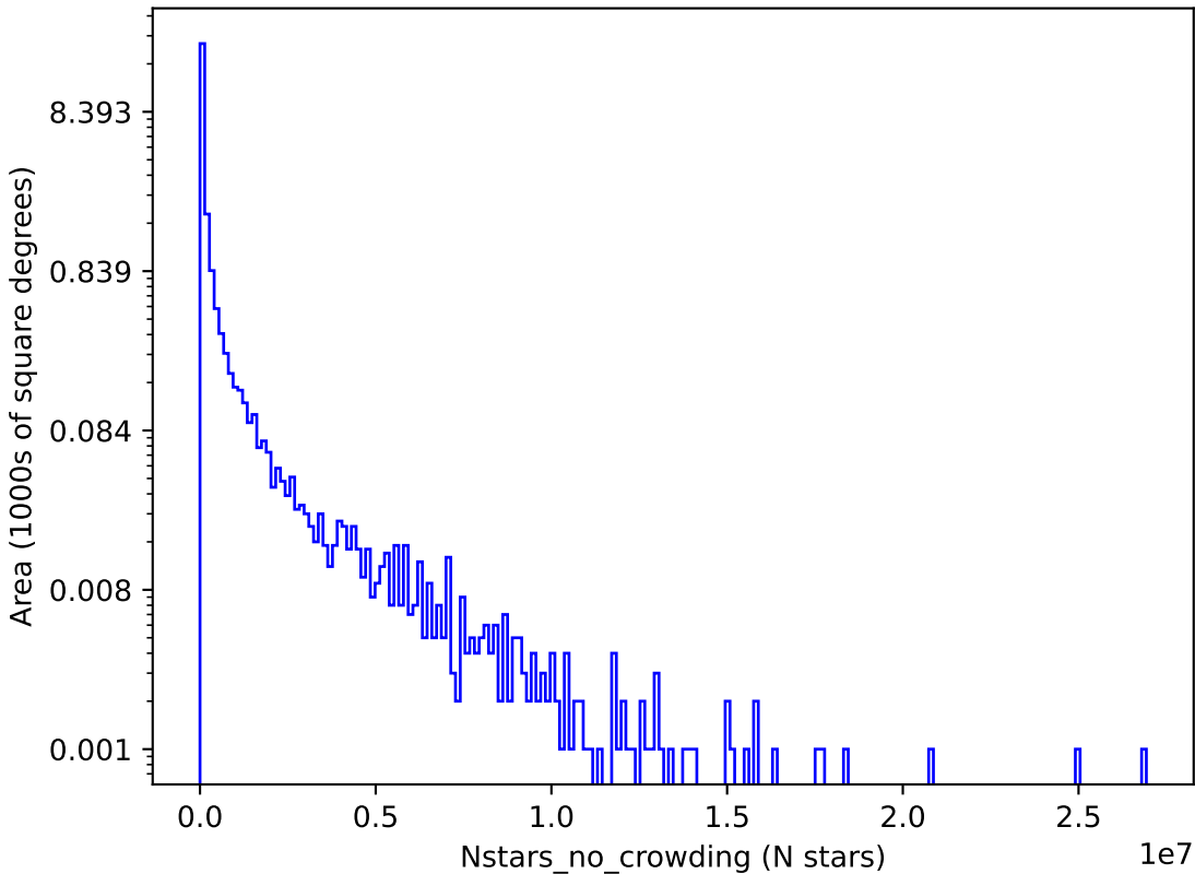
too_elab_r128_d2_griz_v3.4_10yrs i: Nstars_no_crowding
