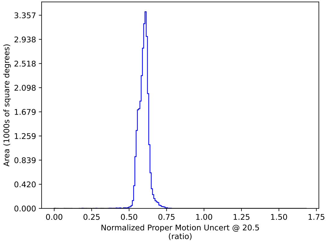
too_elab_r128_d2_griz_v3.4_10yrs : Normalized Proper Motion Uncert @ 20.5
