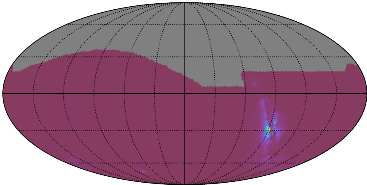
too_elab_r128_d2_griz_v3.4_10yrs : NlcPoints
