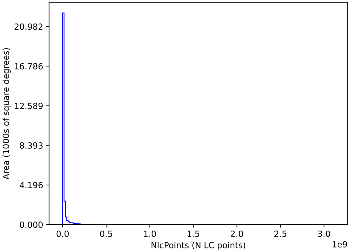
too_elab_r128_d2_griz_v3.4_10yrs : NlcPoints
