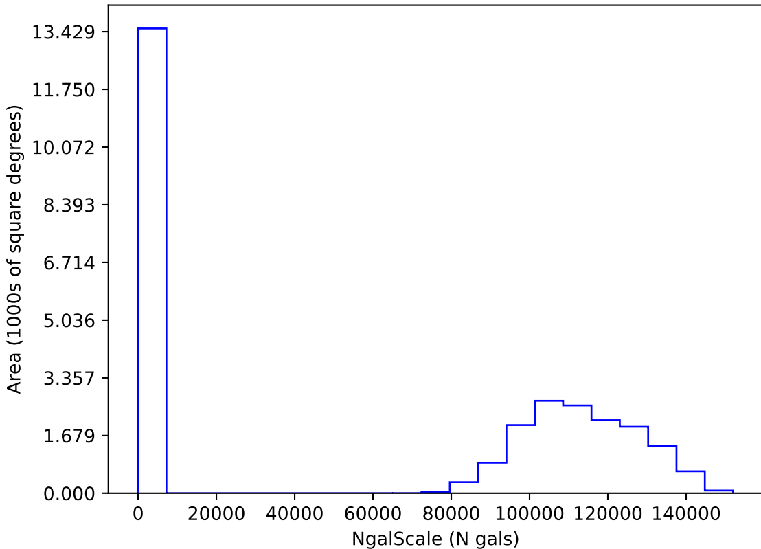
too_elab_r128_d2_griz_v3.4_10yrs i: NgalScale
