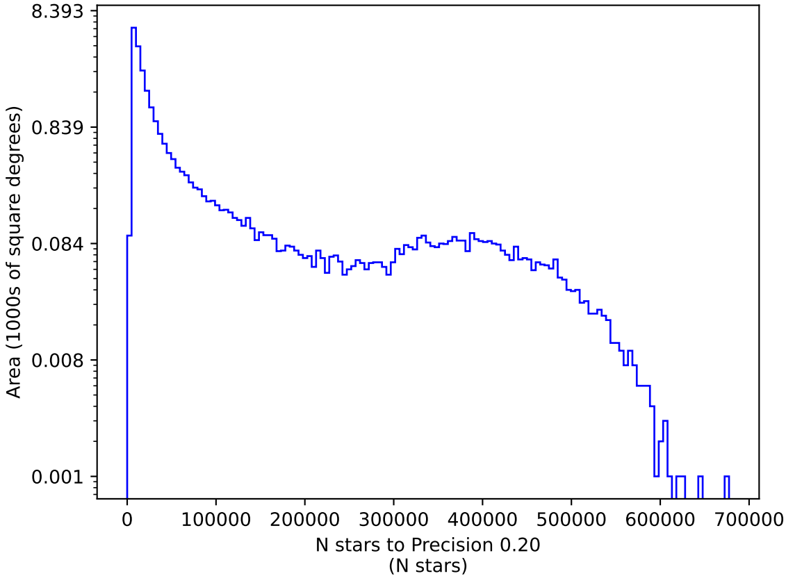
too_elab_r128_d2_griz_v3.4_10yrs z: N stars to Precision 0.20
