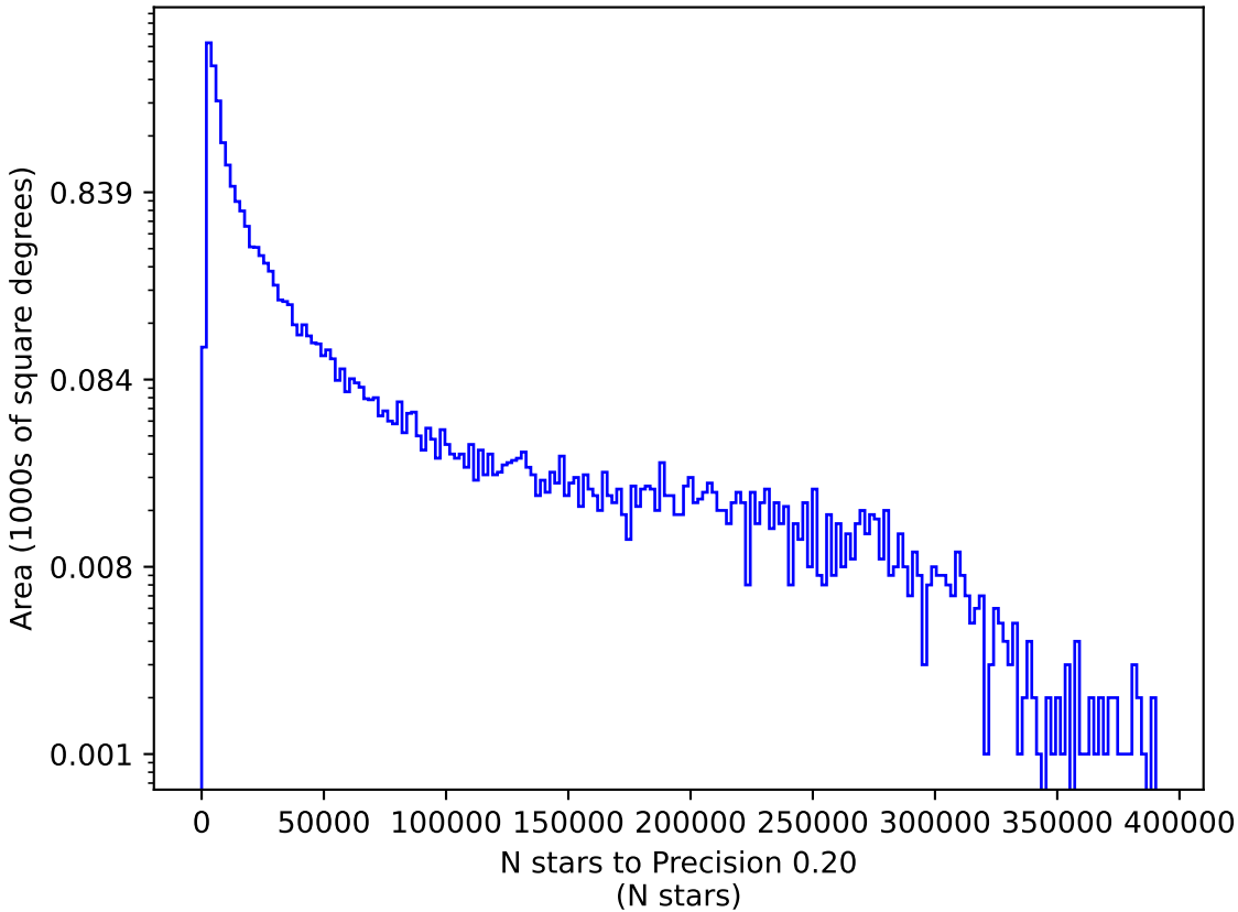
too_elab_r128_d2_griz_v3.4_10yrs u: N stars to Precision 0.20
