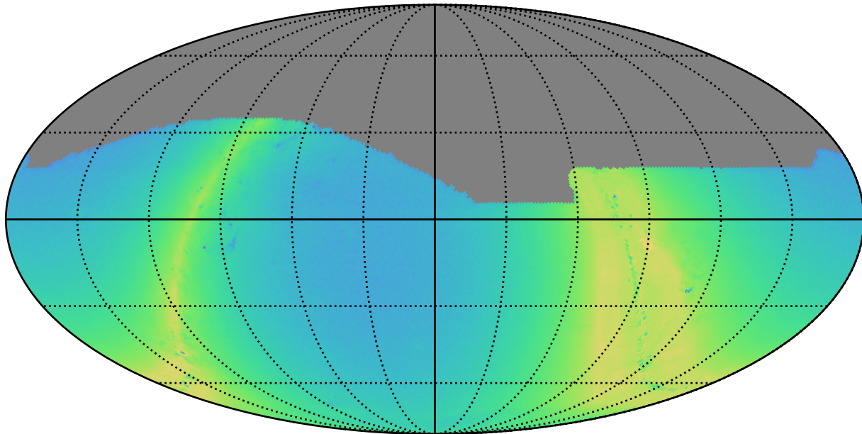
too_elab_r128_d2_griz_v3.4_10yrs r: N stars to Precision 0.20
