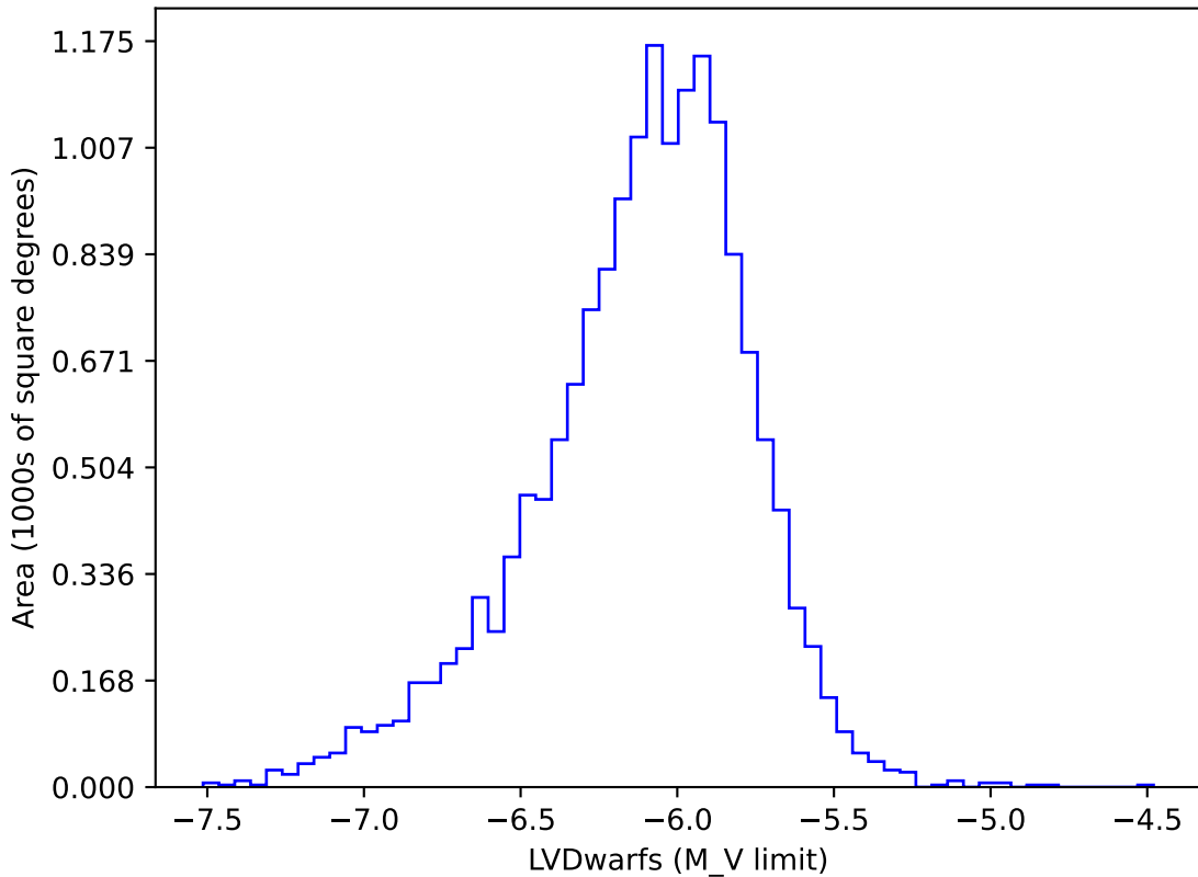
too_elab_r128_d2_griz_v3.4_10yrs gi: LVDwarfs
