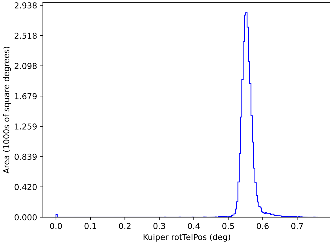
too_elab_r128_d2_griz_v3.4_10yrs y: Kuiper rotTelPos
