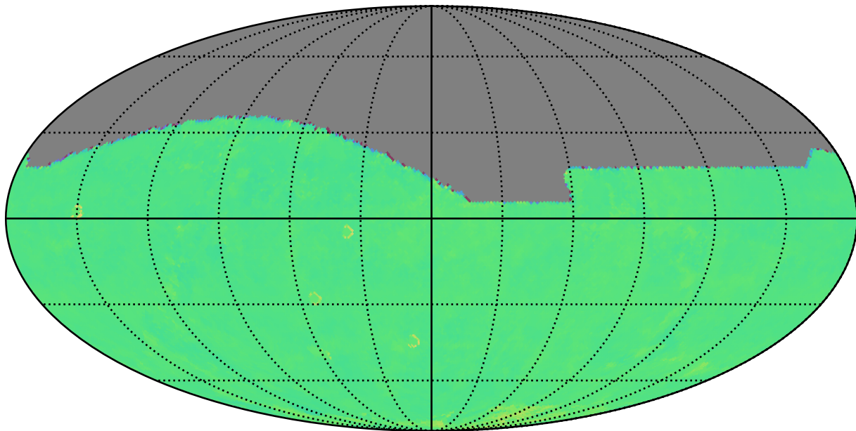
too_elab_r128_d2_griz_v3.4_10yrs r: Kuiper rotTelPos
