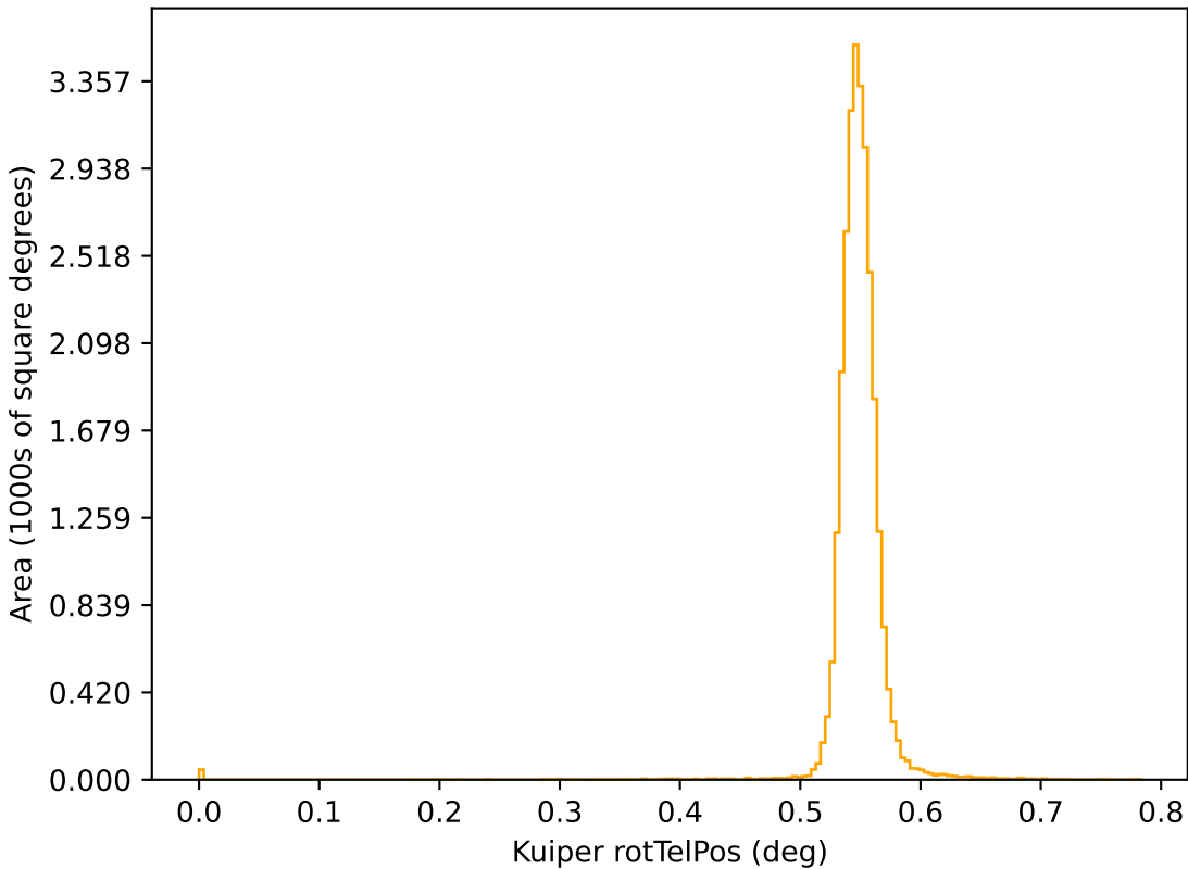
too_elab_r128_d2_griz_v3.4_10yrs r: Kuiper rotTelPos
