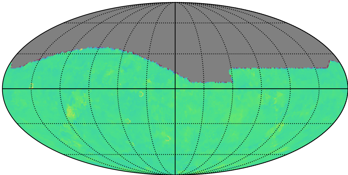
too_elab_r128_d2_griz_v3.4_10yrs g: Kuiper rotTelPos
