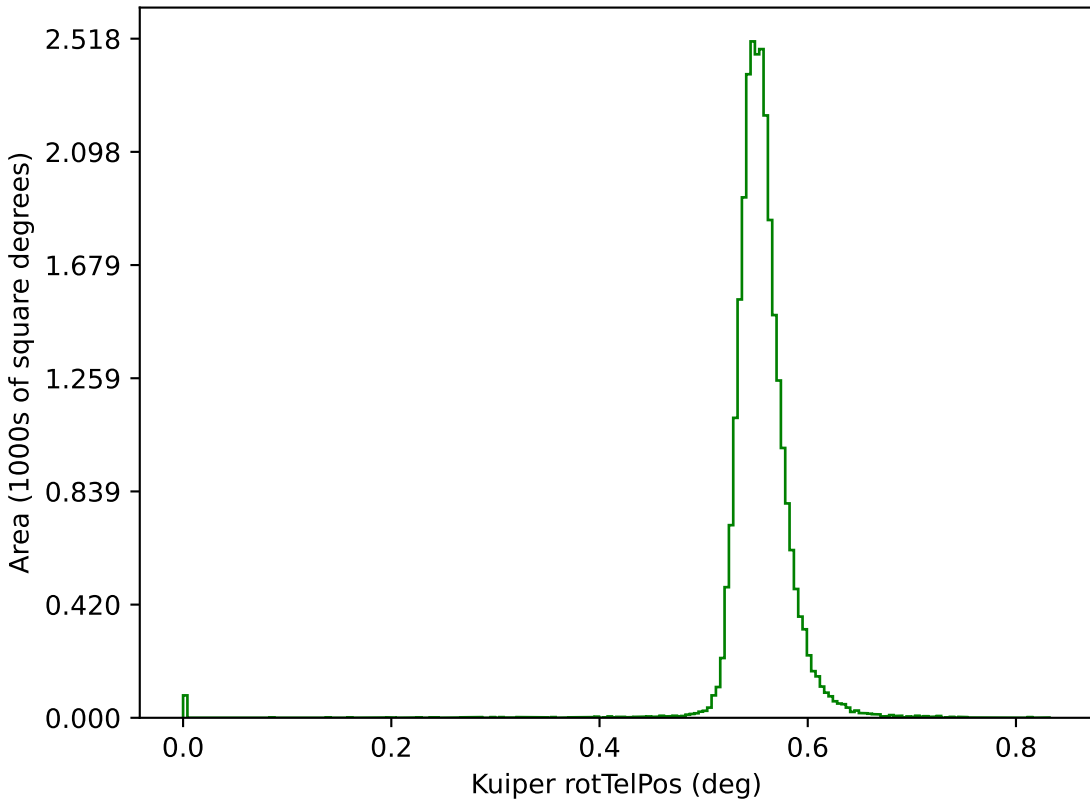
too_elab_r128_d2_griz_v3.4_10yrs g: Kuiper rotTelPos
