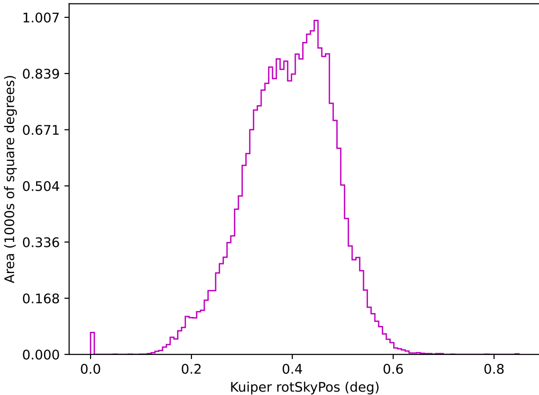
too_elab_r128_d2_griz_v3.4_10yrs z: Kuiper rotSkyPos
