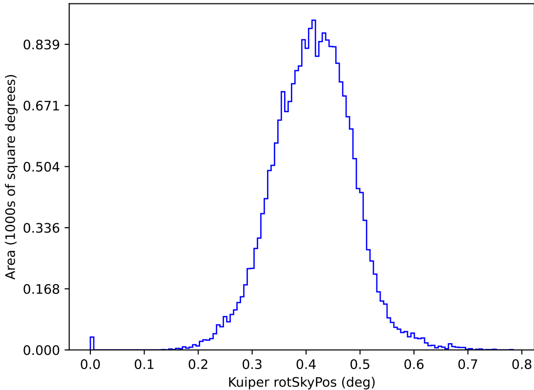
too_elab_r128_d2_griz_v3.4_10yrs y: Kuiper rotSkyPos
