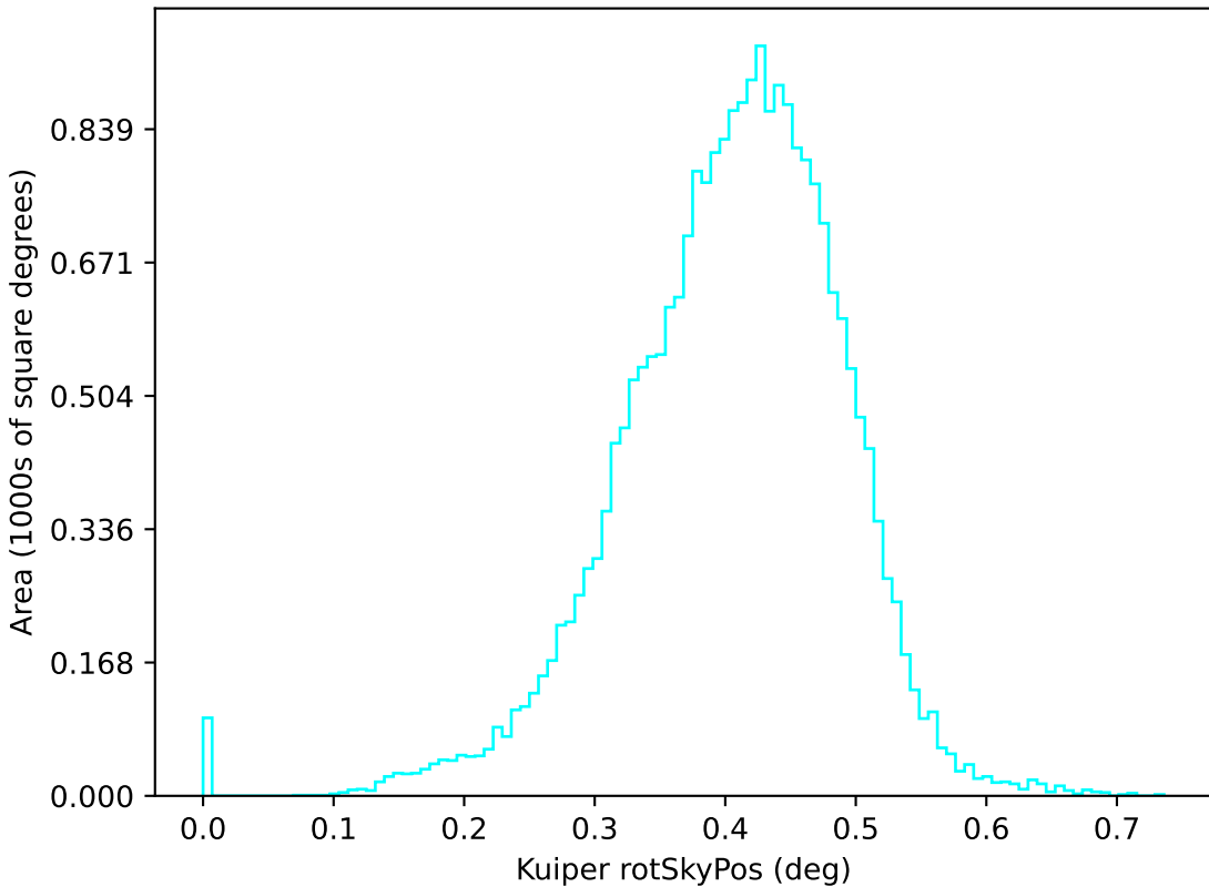
too_elab_r128_d2_griz_v3.4_10yrs u: Kuiper rotSkyPos
