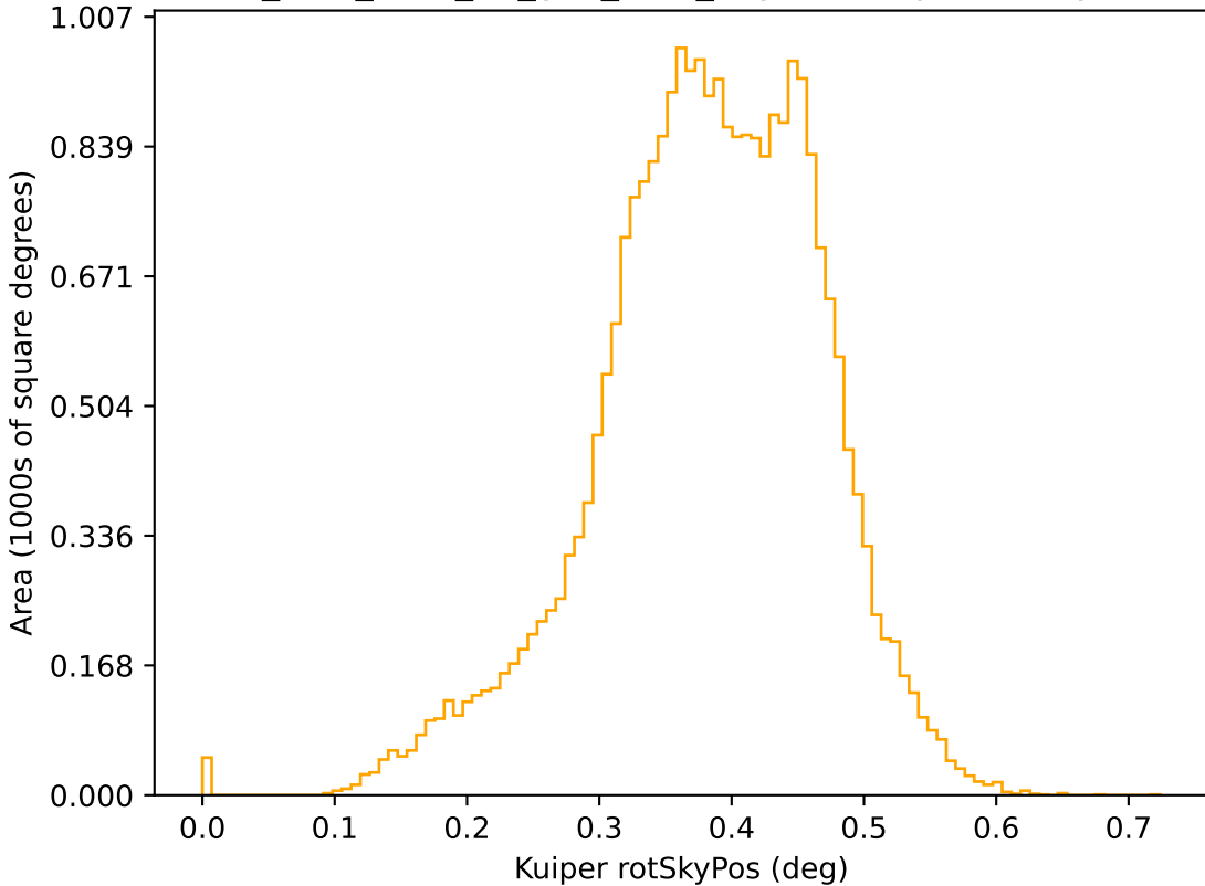
too_elab_r128_d2_griz_v3.4_10yrs r: Kuiper rotSkyPos
