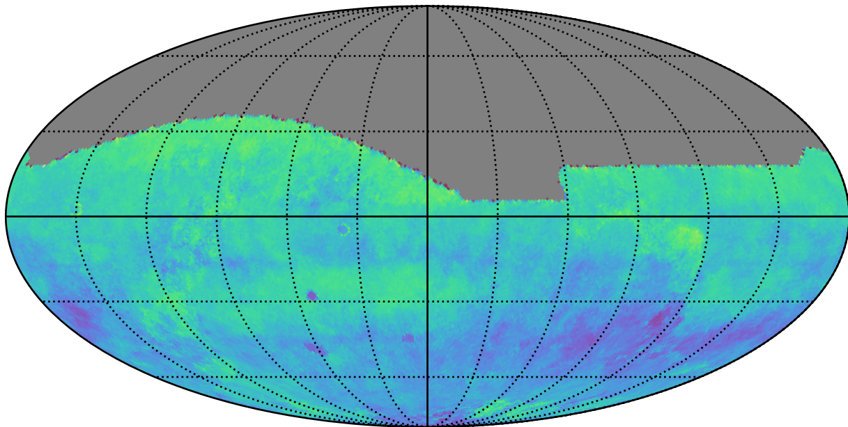
too_elab_r128_d2_griz_v3.4_10yrs i: Kuiper rotSkyPos
