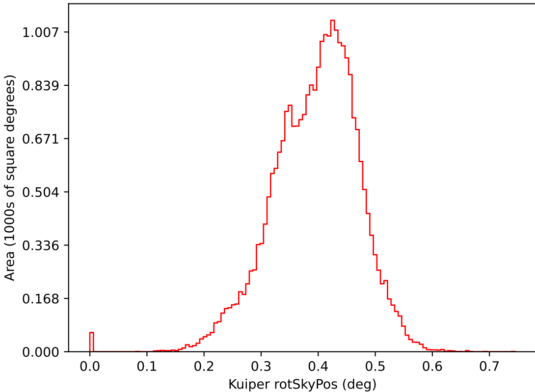
too_elab_r128_d2_griz_v3.4_10yrs i: Kuiper rotSkyPos
