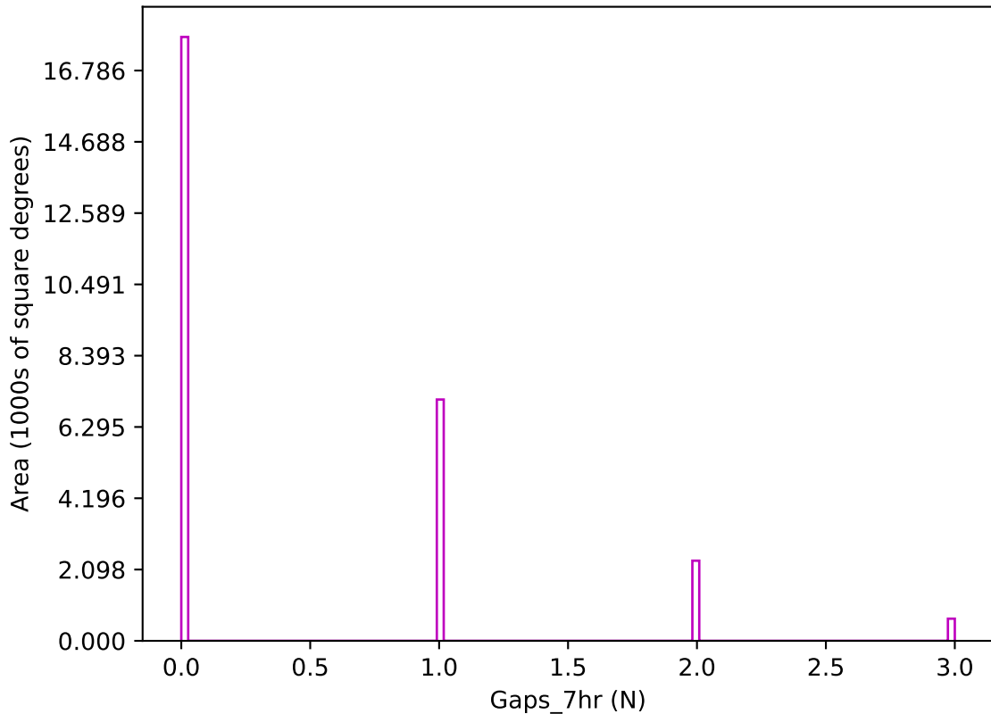
too_elab_r128_d2_griz_v3.4_10yrs z band: Gaps_7hr
