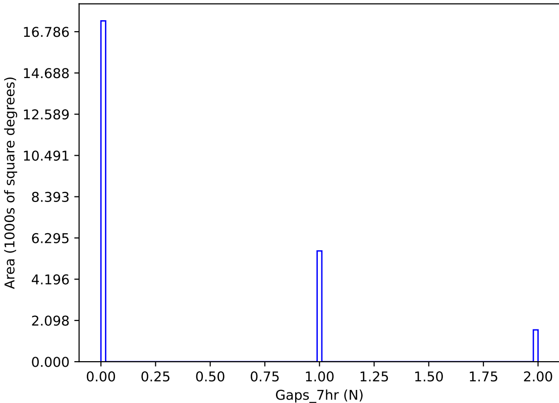
too_elab_r128_d2_griz_v3.4_10yrs y band: Gaps_7hr
