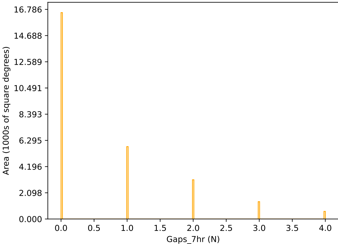
too_elab_r128_d2_griz_v3.4_10yrs r band: Gaps_7hr
