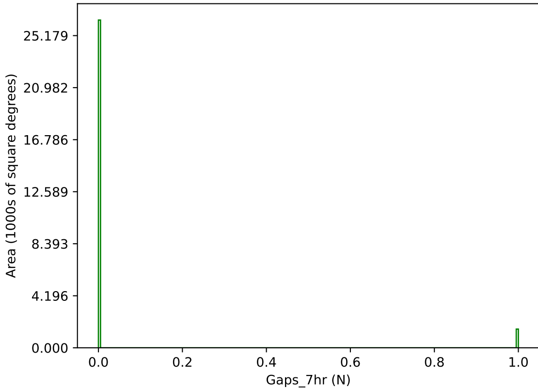
too_elab_r128_d2_griz_v3.4_10yrs g band: Gaps_7hr
