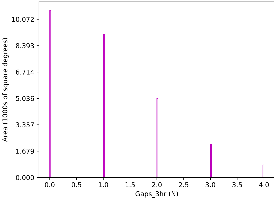
too_elab_r128_d2_griz_v3.4_10yrs z band: Gaps_3hr
