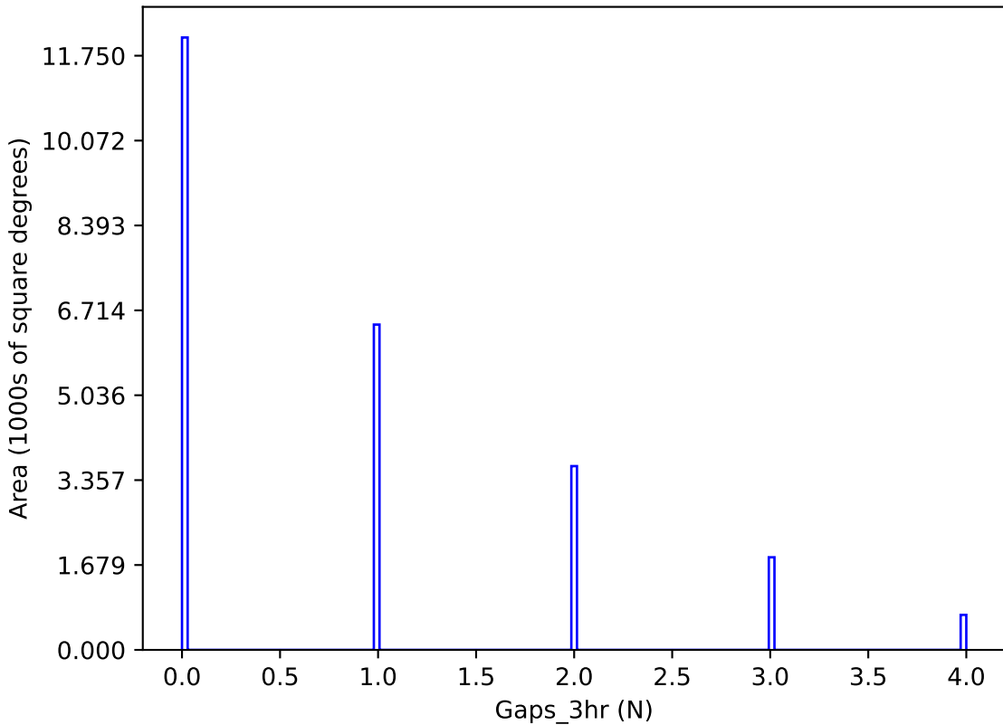
too_elab_r128_d2_griz_v3.4_10yrs y band: Gaps_3hr
