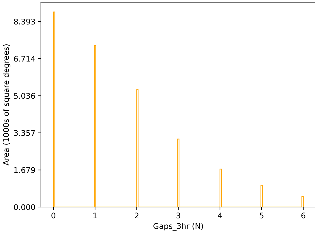
too_elab_r128_d2_griz_v3.4_10yrs r band: Gaps_3hr
