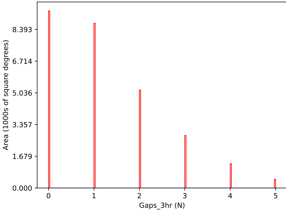
too_elab_r128_d2_griz_v3.4_10yrs i band: Gaps_3hr
