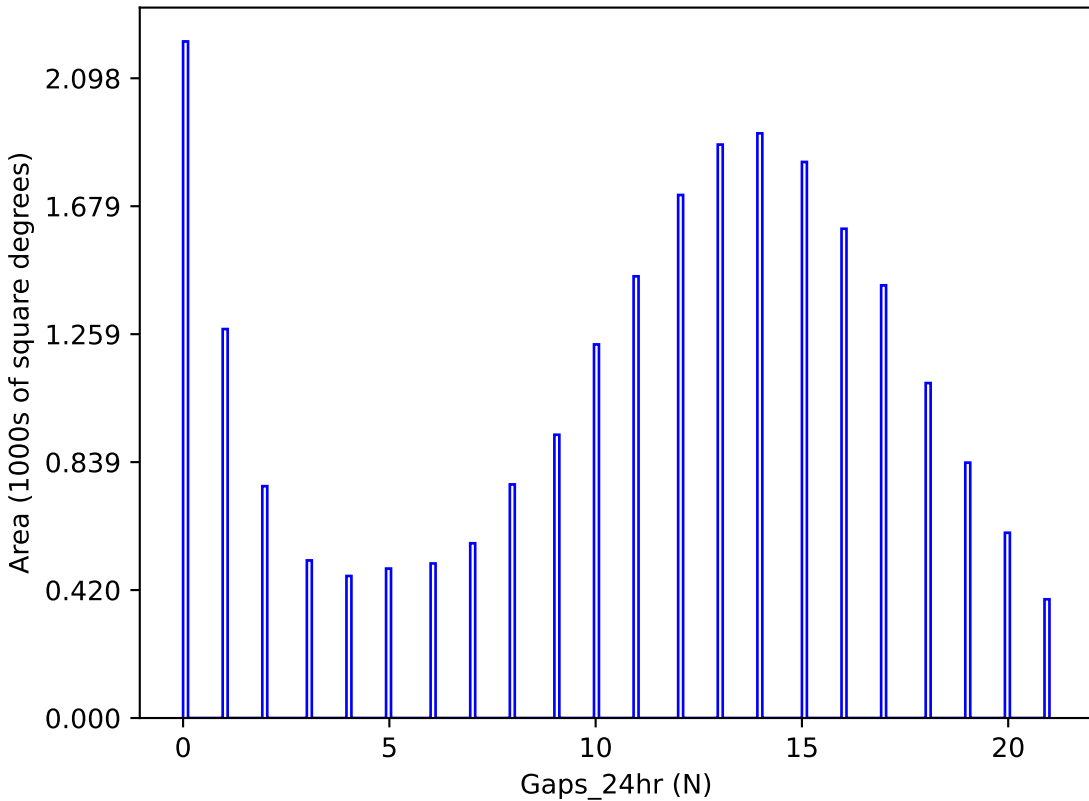
too_elab_r128_d2_griz_v3.4_10yrs y band: Gaps_24hr
