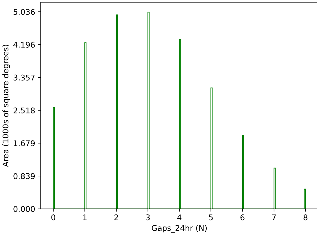
too_elab_r128_d2_griz_v3.4_10yrs g band: Gaps_24hr
