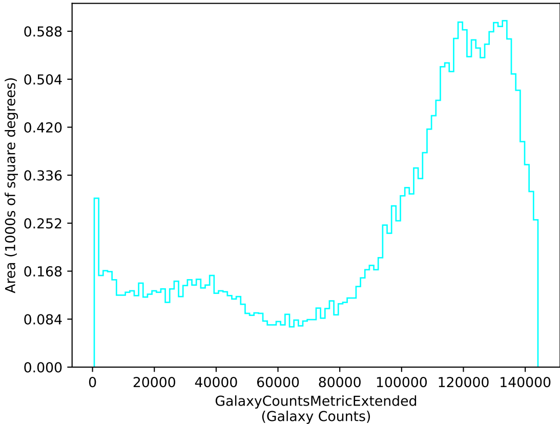
too_elab_r128_d2_griz_v3.4_10yrs u: GalaxyCountsMetricExtended
