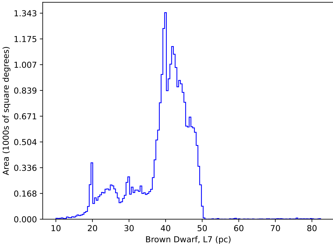
too_elab_r128_d2_griz_v3.4_10yrs : Brown Dwarf, L7
