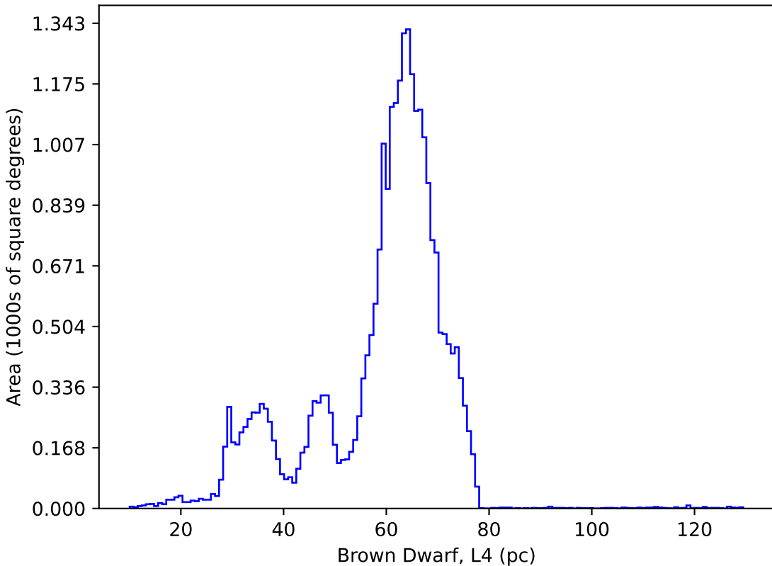
too_elab_r128_d2_griz_v3.4_10yrs : Brown Dwarf, L4
