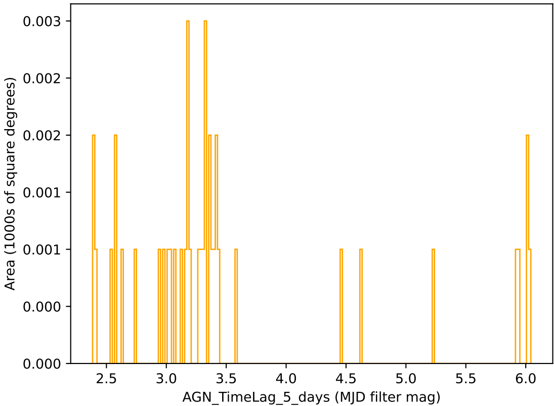
too_elab_r128_d2_griz_v3.4_10yrs r band: AGN_TimeLag_5_days
